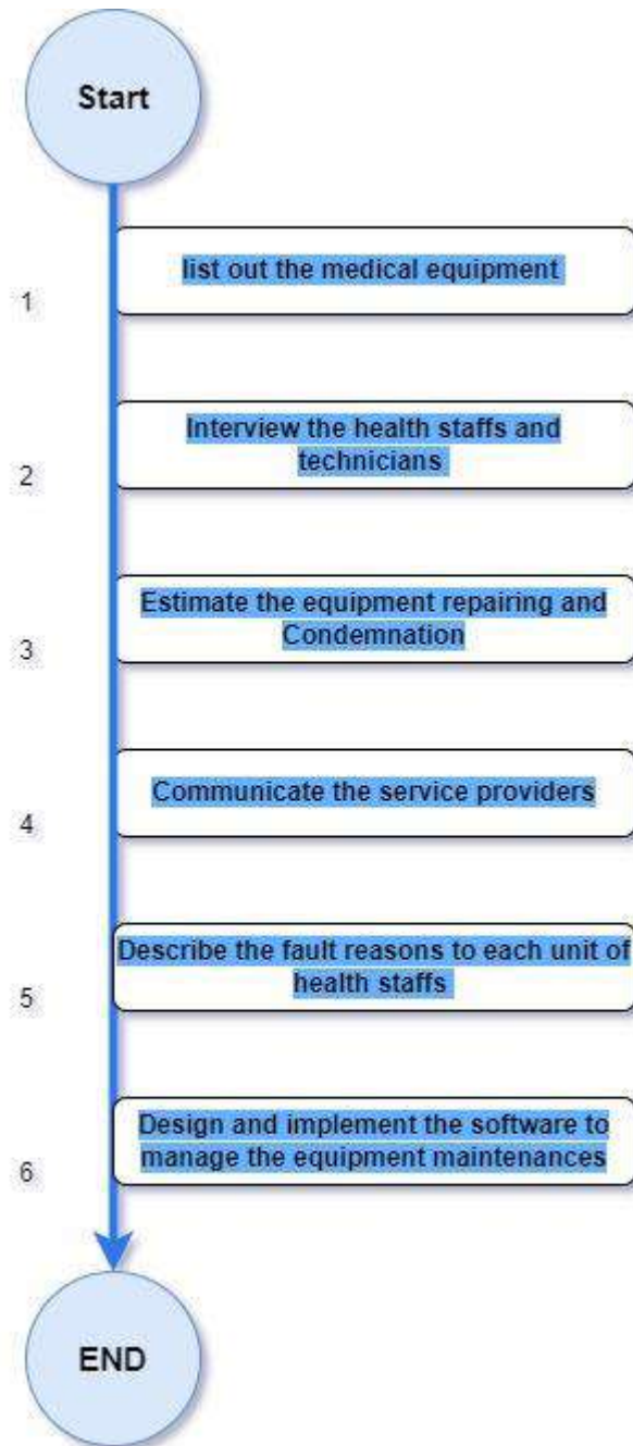
Figure 1: Methodology diagram.
